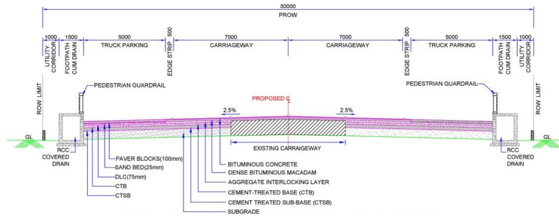
TCS-III: 4 LANE UNDIVIDED CARRIAGEWAY WITH TRUCK PARKING (EXISTING ROAD) (AS PER IRC SP-63 2004)
