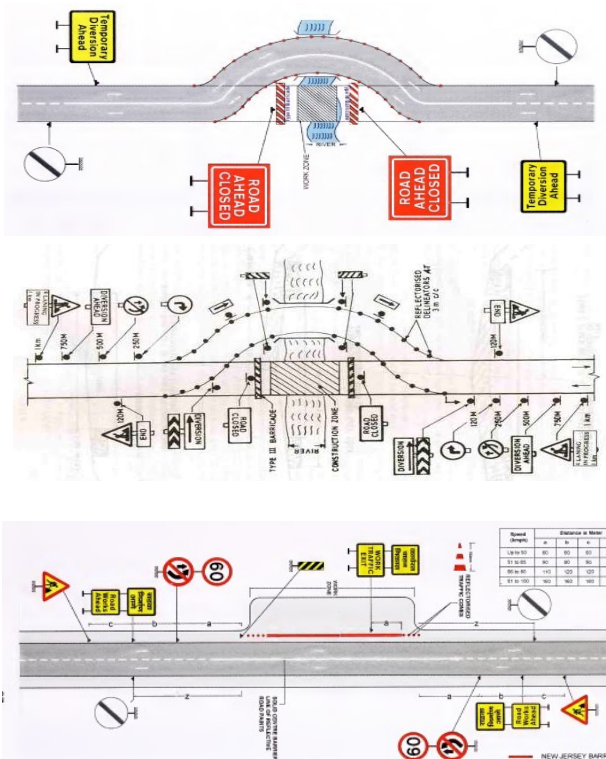
Fig. 10.1 Two Lane to Four Lane (Eccentric Widening)
