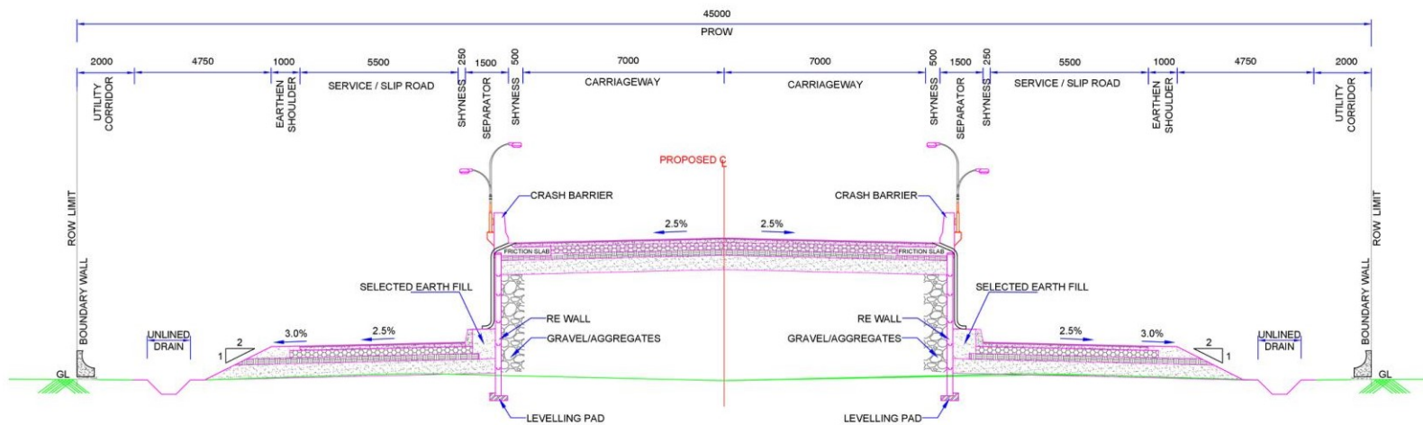
TCS-IV : 4 LANE DIVIDED CARRIAGEWAY FOR APPROACHES TO VUP WITH SLIP ROADS ON BOTH SIDES
